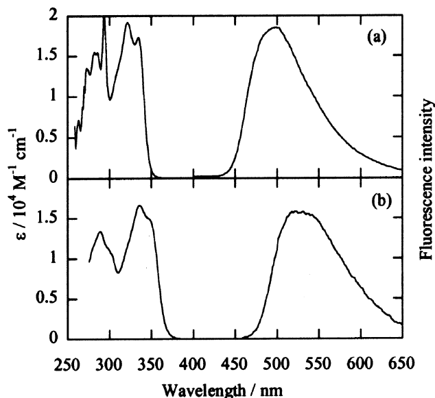
Fig. 3 Absorption and fluorescence spectra of HBO (a) and HBT (b) in benzene.
