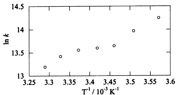
Fig. 5 Arrhenius plot for decay constants of HBO tautomer in methylcyclohexane.
