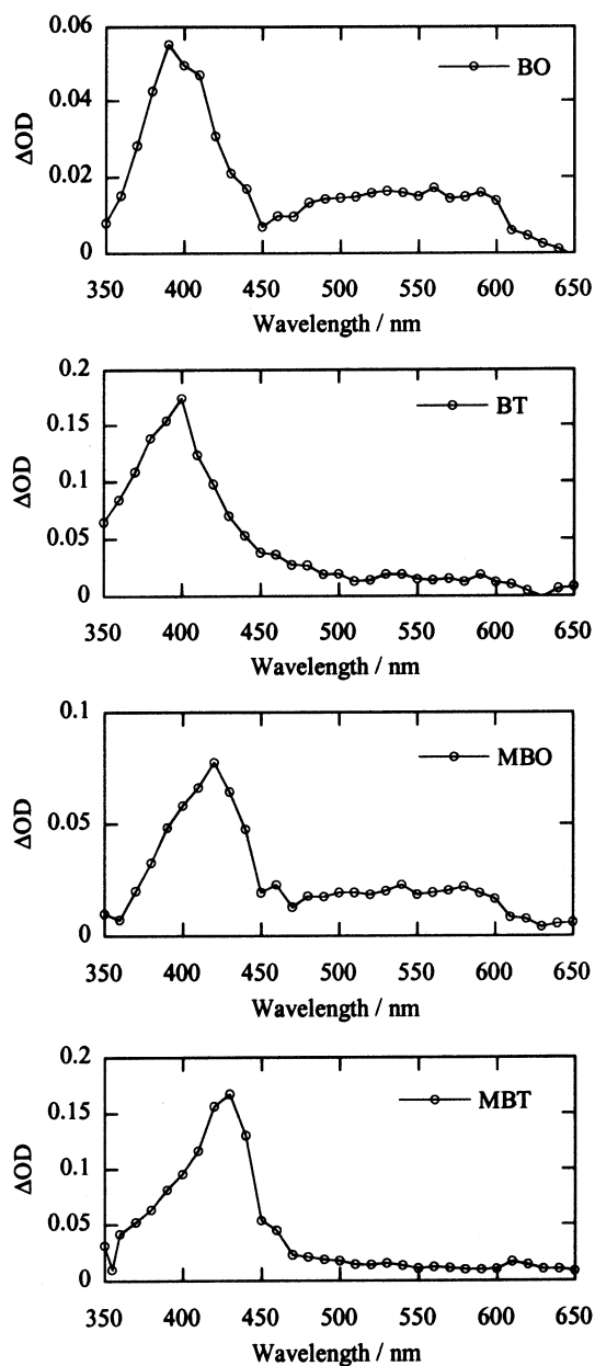
Fig. 9 Transient absorption spectra of BO, BT, MBO and MBT in benzene.
