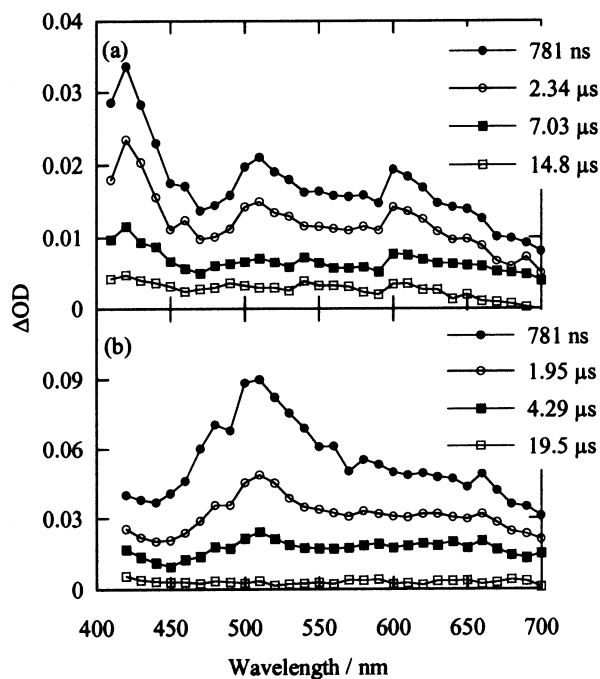
Fig. 10 Transient absorption spectra of HBO (a) and HBT (b) on triplet sensitization in benzene.
