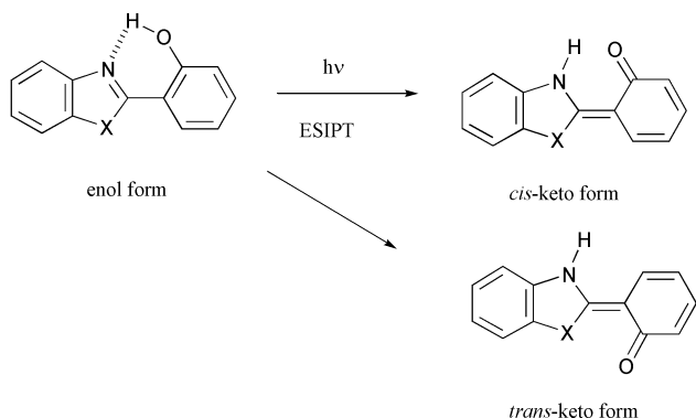
Fig. 2 Excited state intramolecular hydrogen atom transfer of HBO and HBT.
