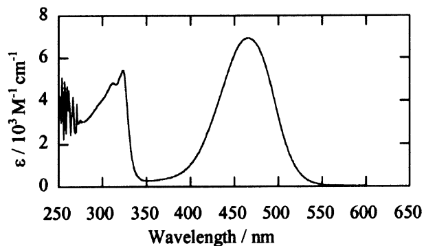
Fig. 6 Absorption spectrum of trans -NBT in benzene at room temperature.
