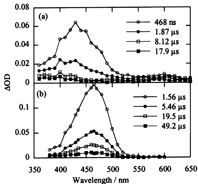
Fig. 4 Transient absorption spectra of HBO (a) and HBT (b) in benzene on direct irradiation.
