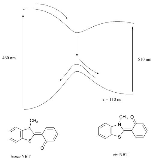
Fig. 11 Potential energy surfaces of isomerization of trans -NBT in benzene at room temperature.
