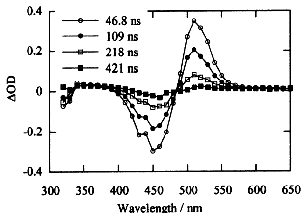
Fig. 7 Transient absorption spectra of trans -NBT in benzene at room temperature.
