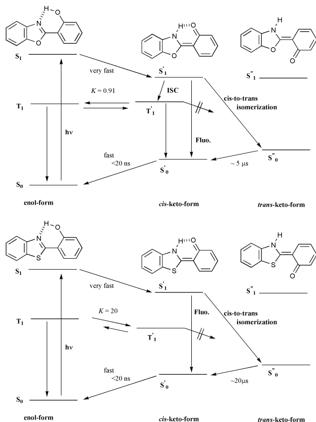
Fig. 12 Energy diagram of hydrogen atom transfer of HBO (above) and HBT (below).
