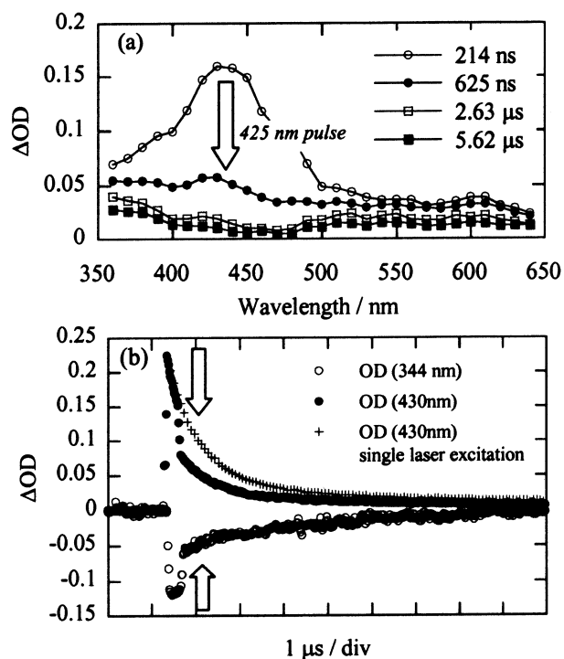
Fig. 8 Transient absorption spectra (a) and time profiles (b) observed by two step laser excitation (308 and 425 nm) monitored at 344 (○) and 430 nm (●) and by single laser excitation (308 nm) monitored at 430 nm (+) of HBO in benzene.
